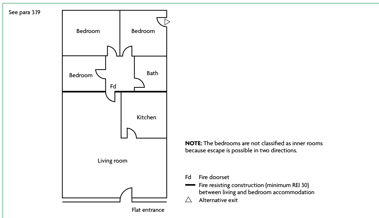
Diagram 3.4 Flat with an alternative exit, but where all habitable rooms have no direct access to an entrance hall
