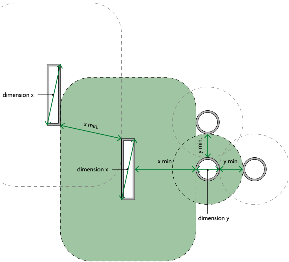
Ceiling plan
