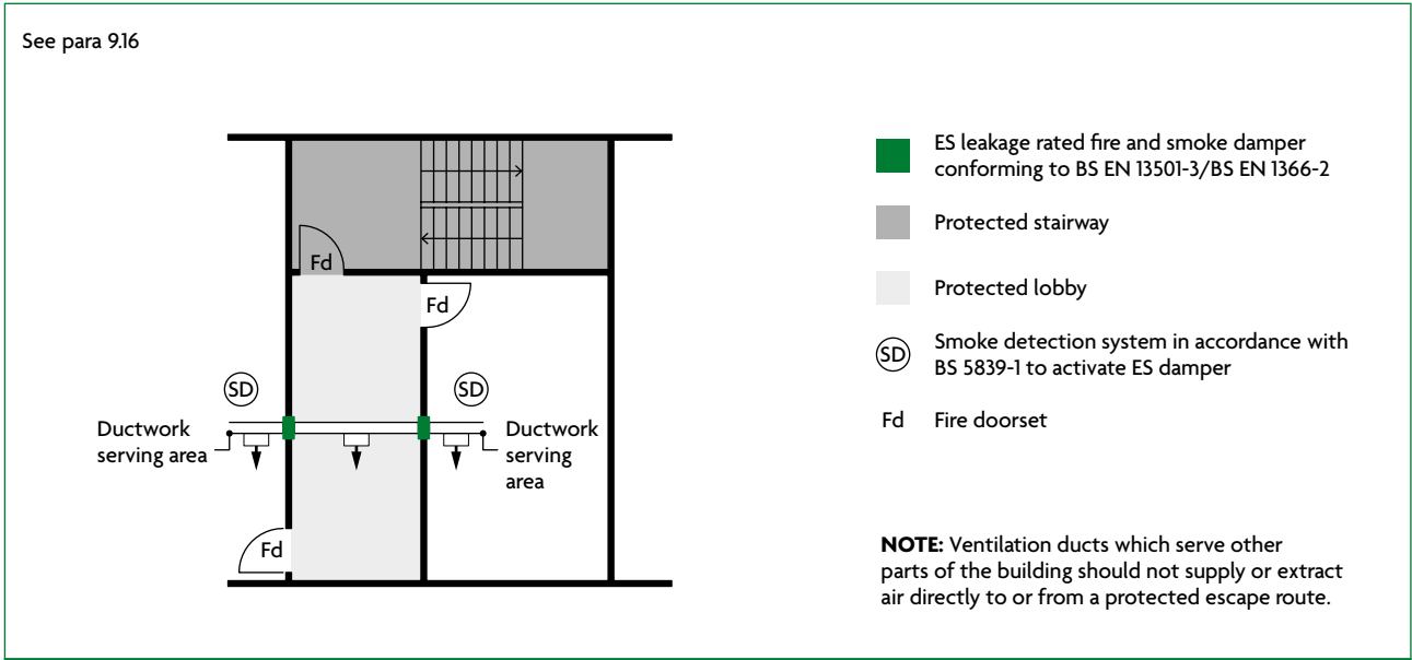
Diagram 9.4 Ductwork passing through protected escape routes – method 4
