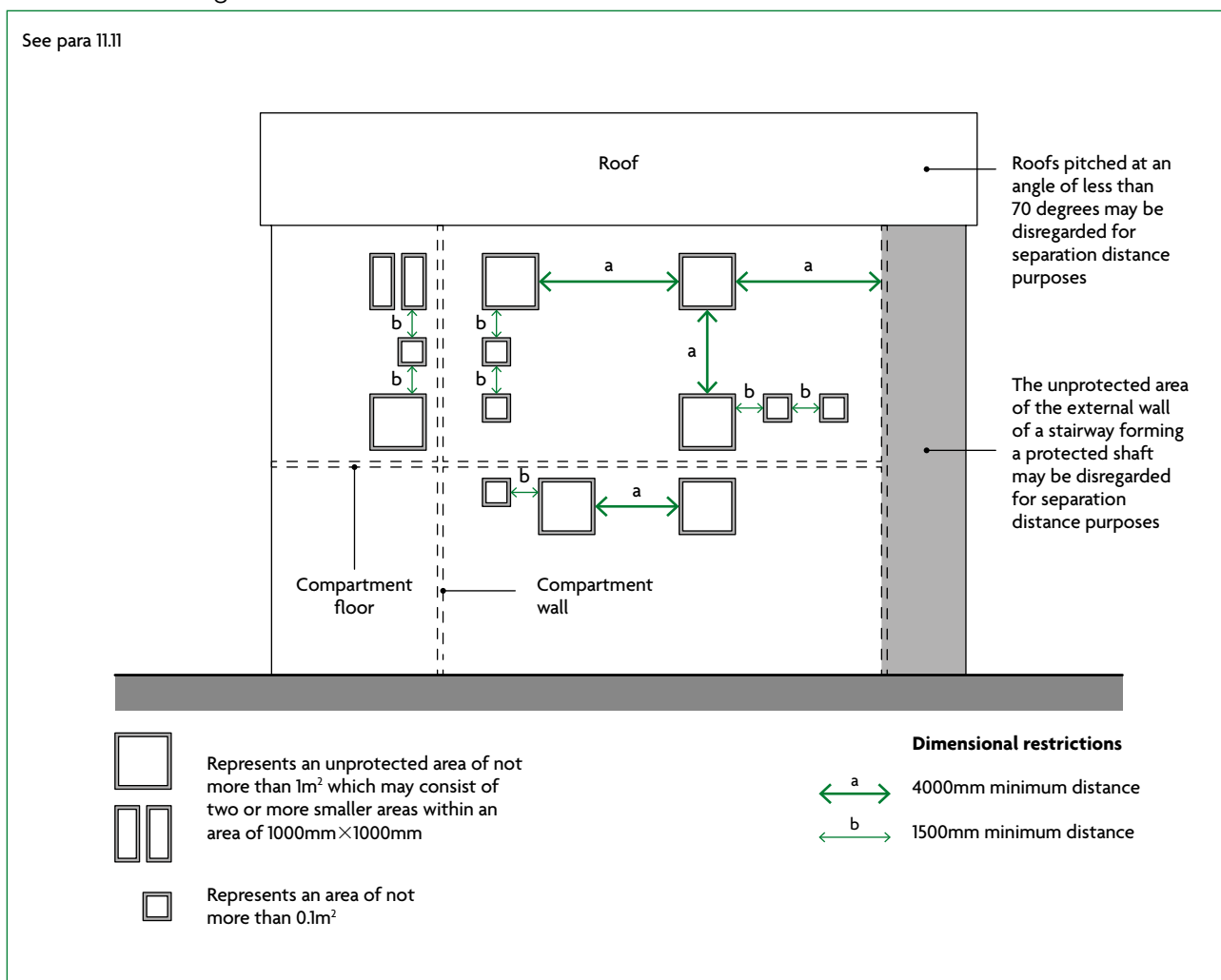
Diagram 11.5 Small unprotected areas that may be disregarded in assessing the separation distance from the boundary
