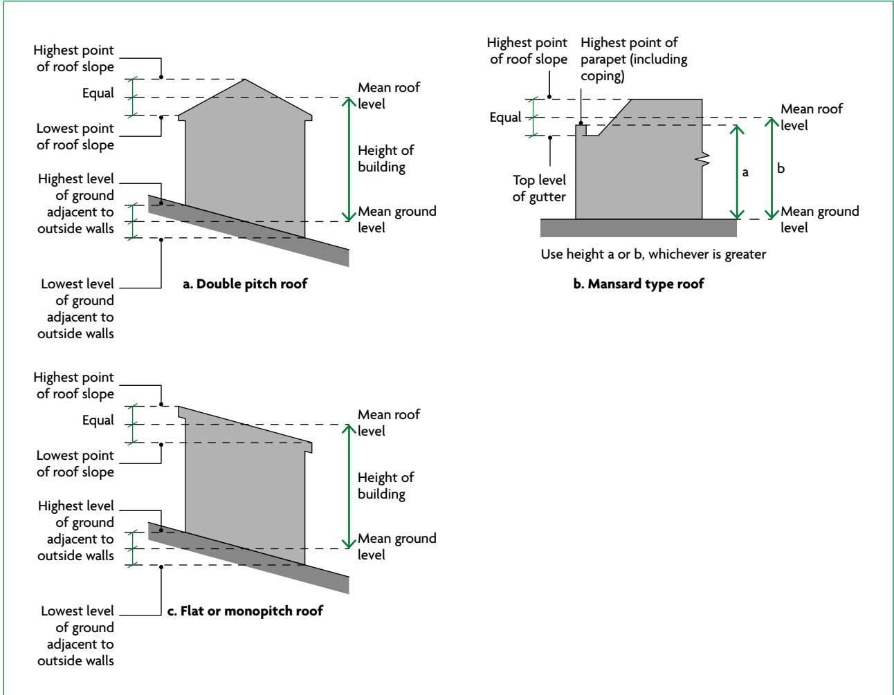
Diagram D4 Height of building
