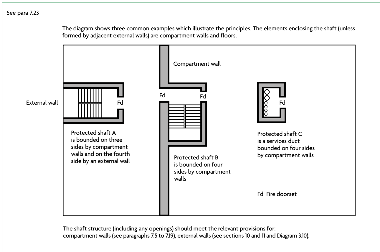
Diagram 7.1 Construction of protected shafts
