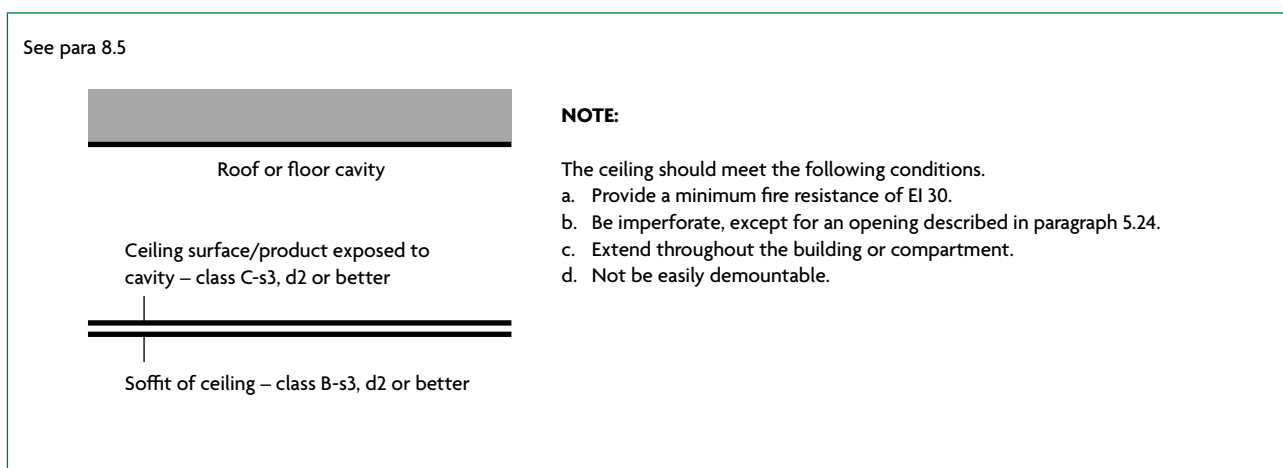
Diagram 8.3 Fire resisting ceiling below concealed space
