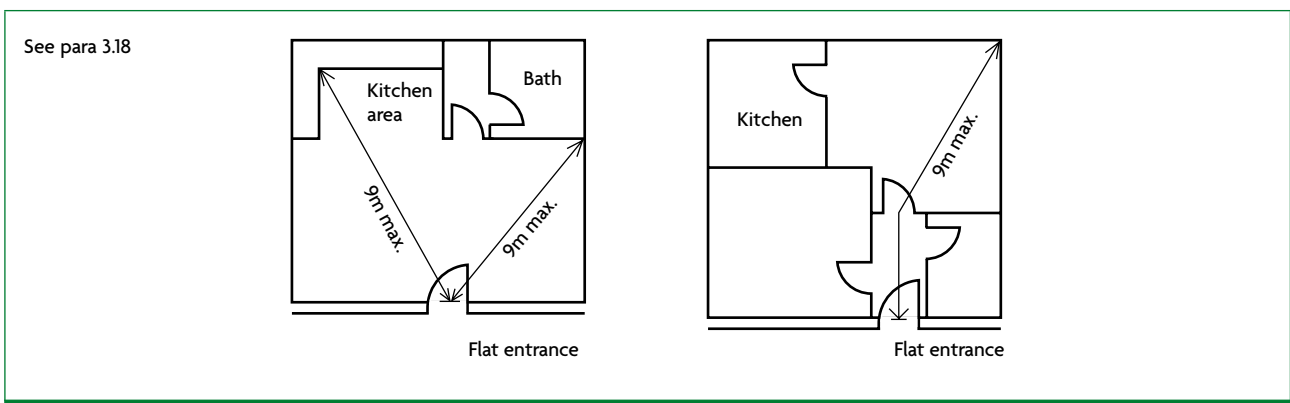
Diagram 3.3 Flat with restricted travel distance from furthest point to entrance
