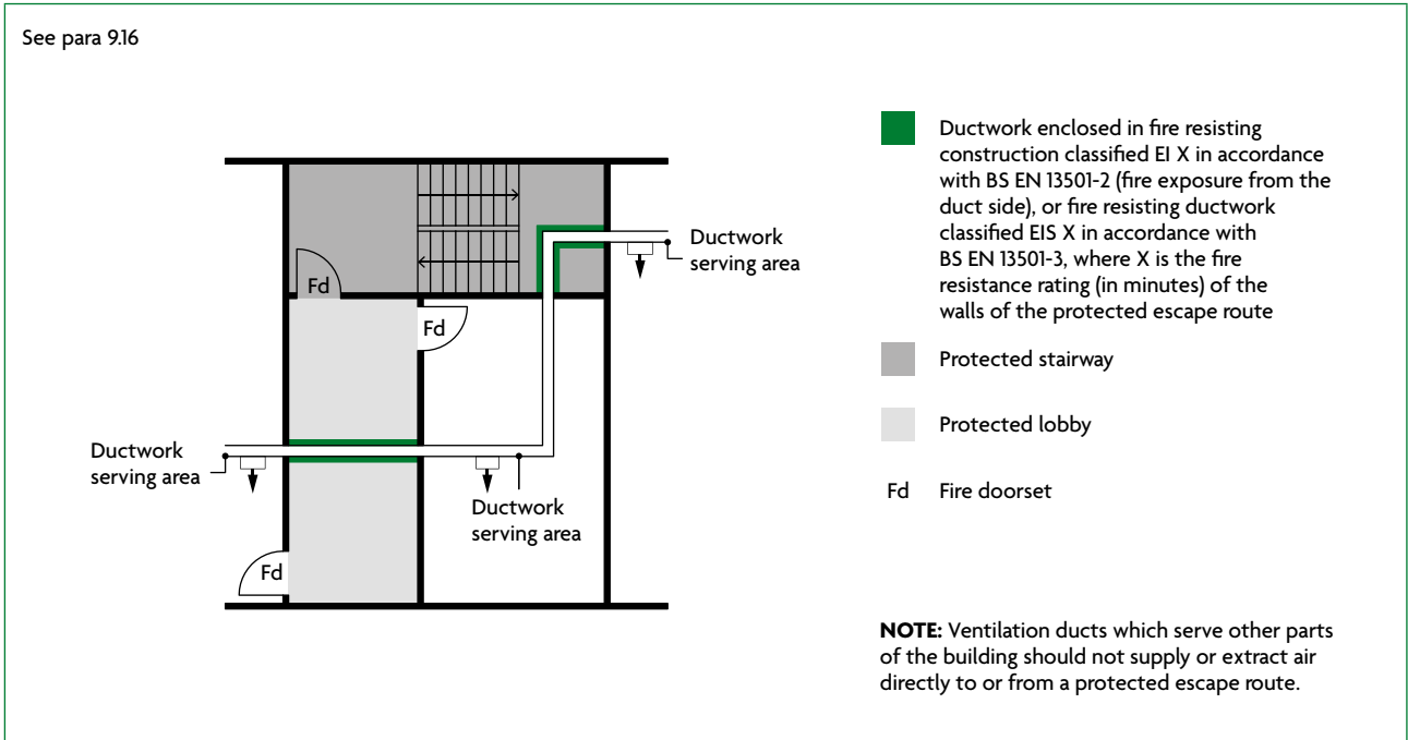
Diagram 9.3 Ductwork passing through protected escape routes – method 2 or method 3
